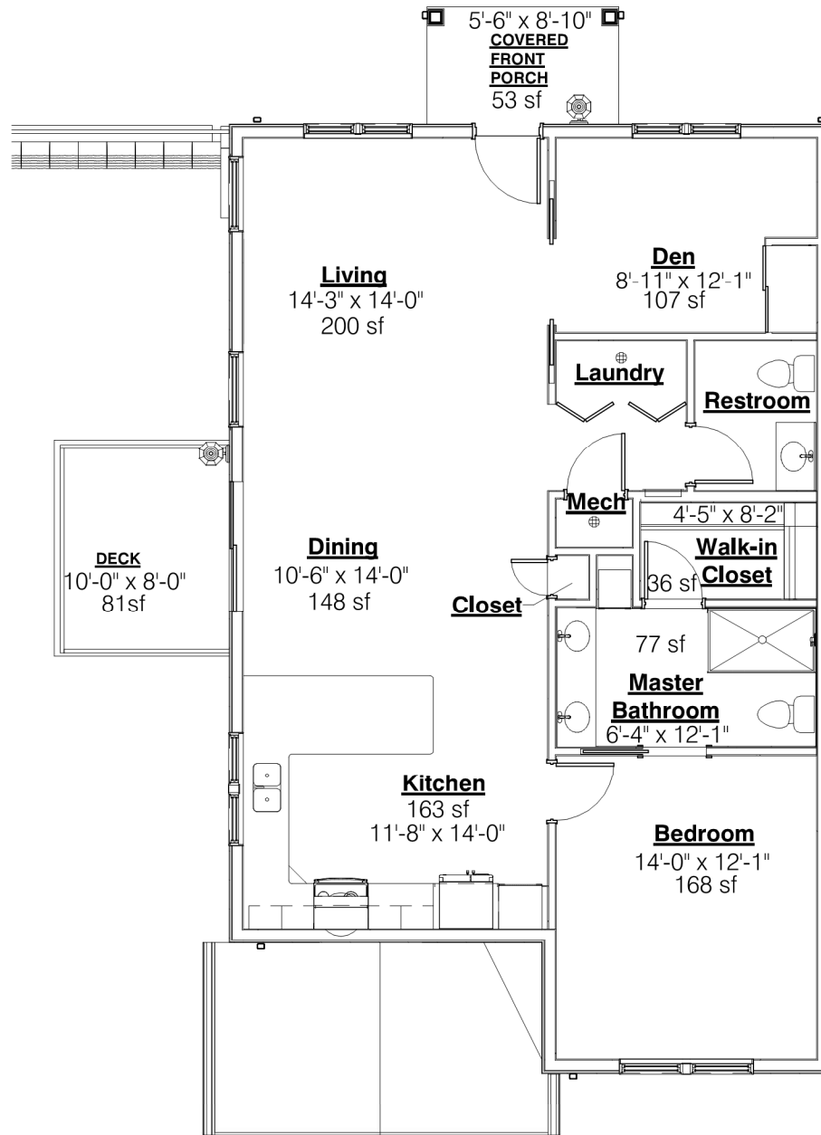
1 | Typical Patio Home - Upper Level - 1,031 SF
