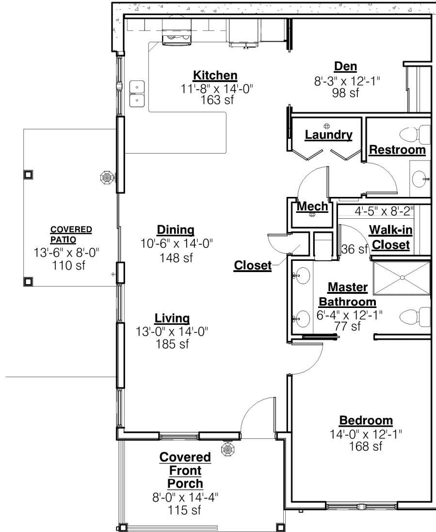
1 Typical Patio Home - Lower Level - 1,022 SF
