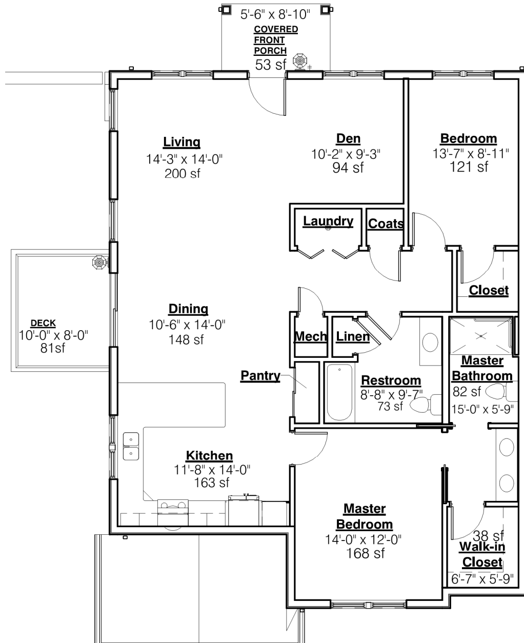
1 Two Bedroom Patio Home - 1,291 SF
